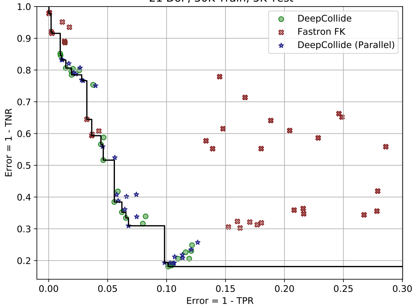
TPR vs. TNR: 21 DoF, 30K Train, 5K Test
